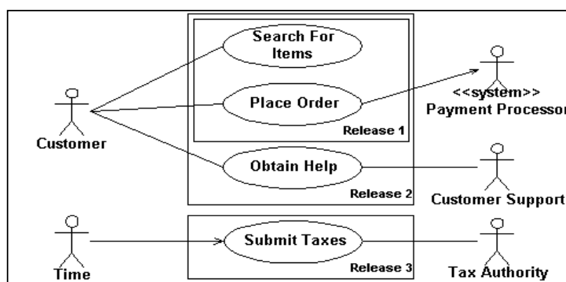
Gambar 5. Contoh use case diagram UML
