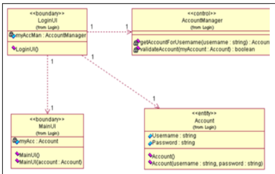
Gambar 8. Contoh notasi class diagram UML
