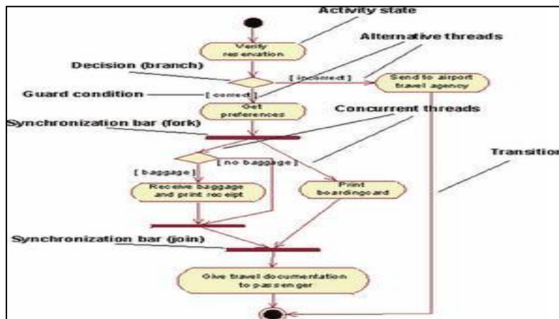
Gambar 6. Contoh activity diagram UML
