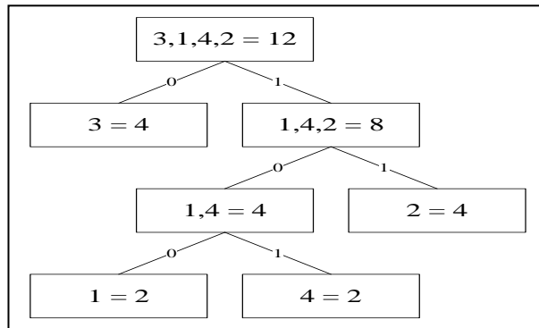
Gambar 10. Penelusuran nilai piksel pohon huffman
