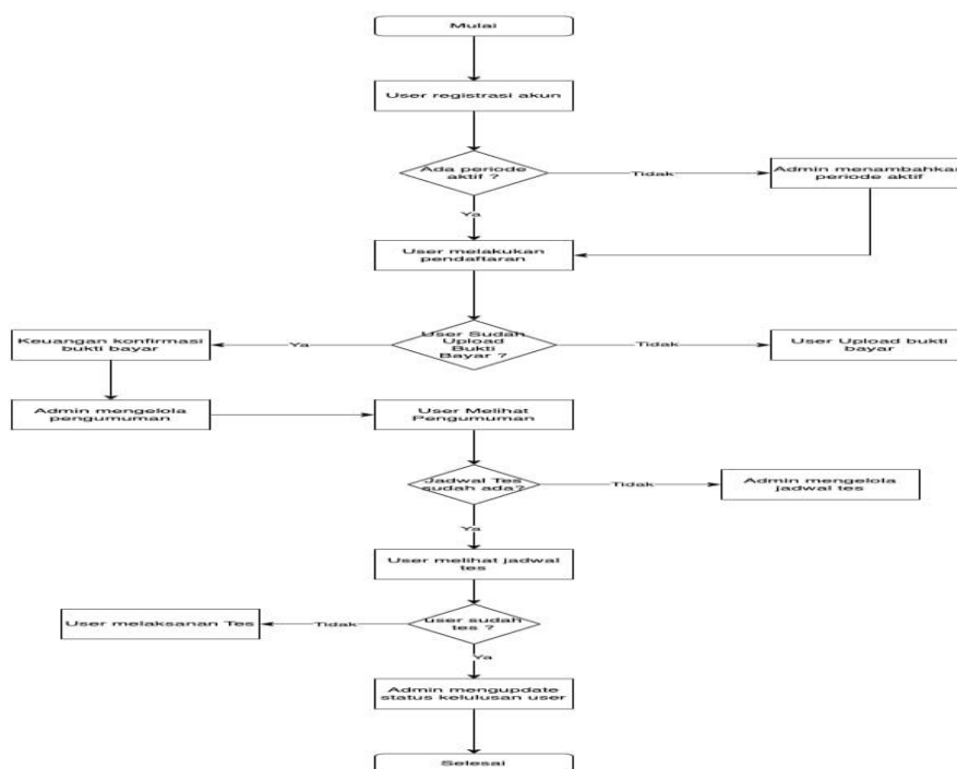
Gambar 4. Flowchart Sistem Berbasis Online
