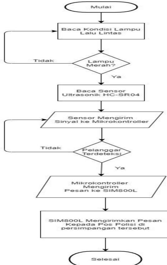
Gambar 6. Flowchart Proses
